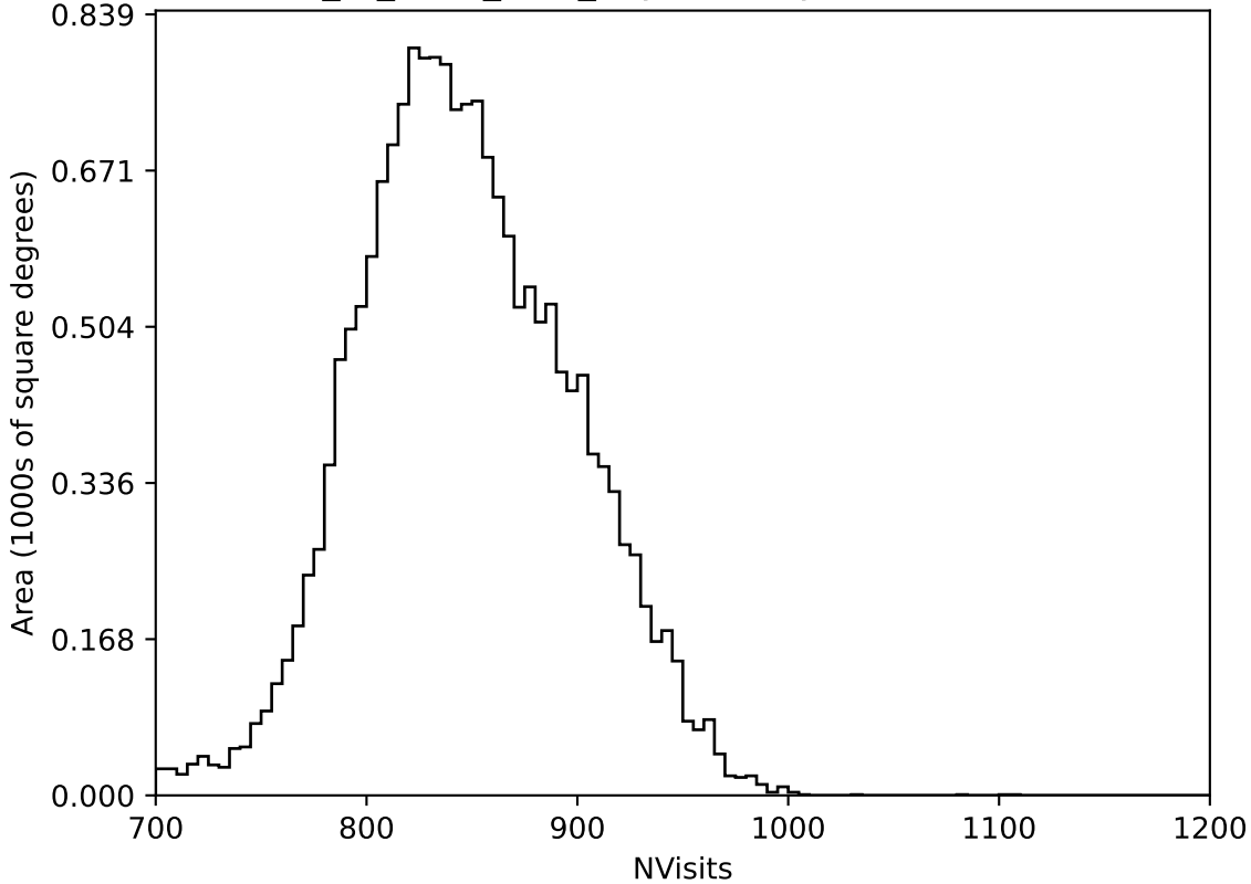
extra_ss_neo2_v3.4_10yrs All sky all bands: NVisits
