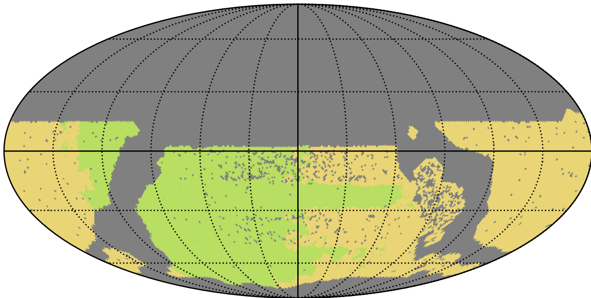
extra_ss_neo2_v3.4_10yrs WFD all bands: NSeasons
