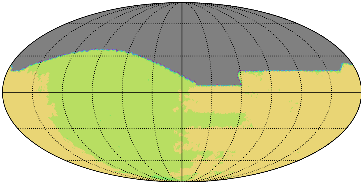
extra_ss_neo2_v3.4_10yrs All sky all bands: NSeasons
