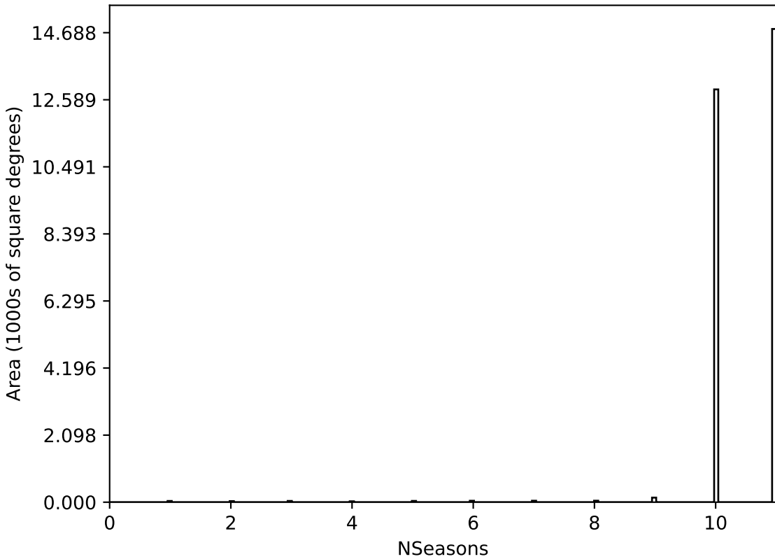
extra_ss_neo2_v3.4_10yrs All sky all bands: NSeasons
