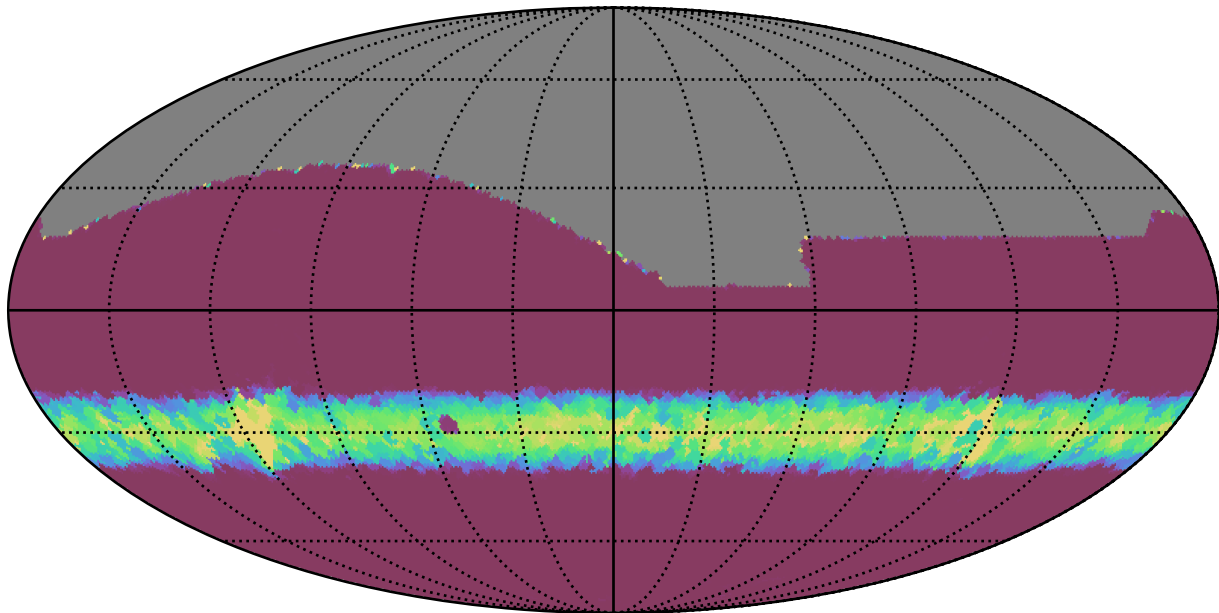
extra_ss_neo2_v3.4_10yrs All sky all bands: Min normairmass
