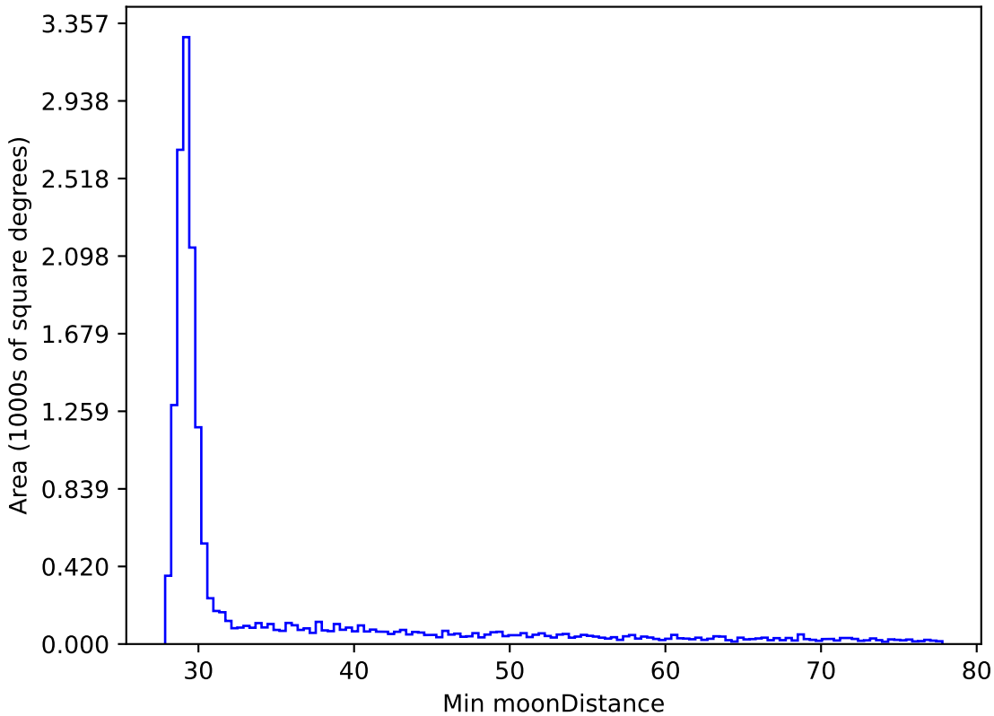
extra_ss_neo2_v3.4_10yrs WFD all bands: Min moonDistance
