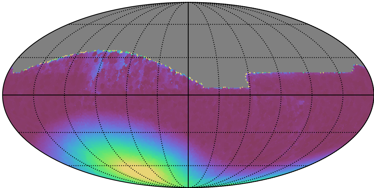
extra_ss_neo2_v3.4_10yrs All sky all bands: Min moonDistance
