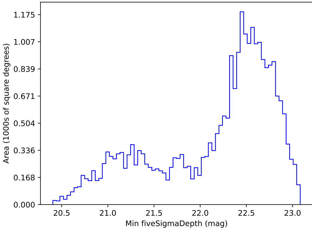
extra_ss_neo2_v3.4_10yrs Yr 1 z band: Min fiveSigmaDepth
