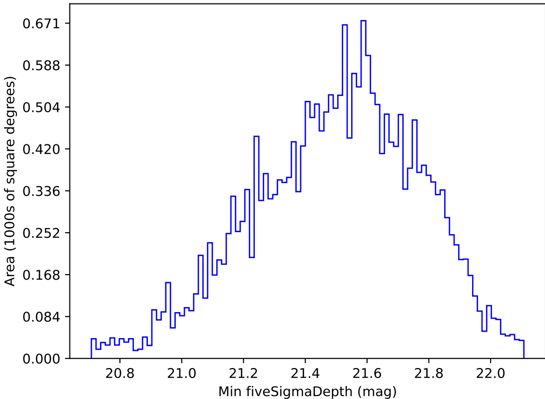
extra_ss_neo2_v3.4_10yrs Yr 1 y band: Min fiveSigmaDepth
