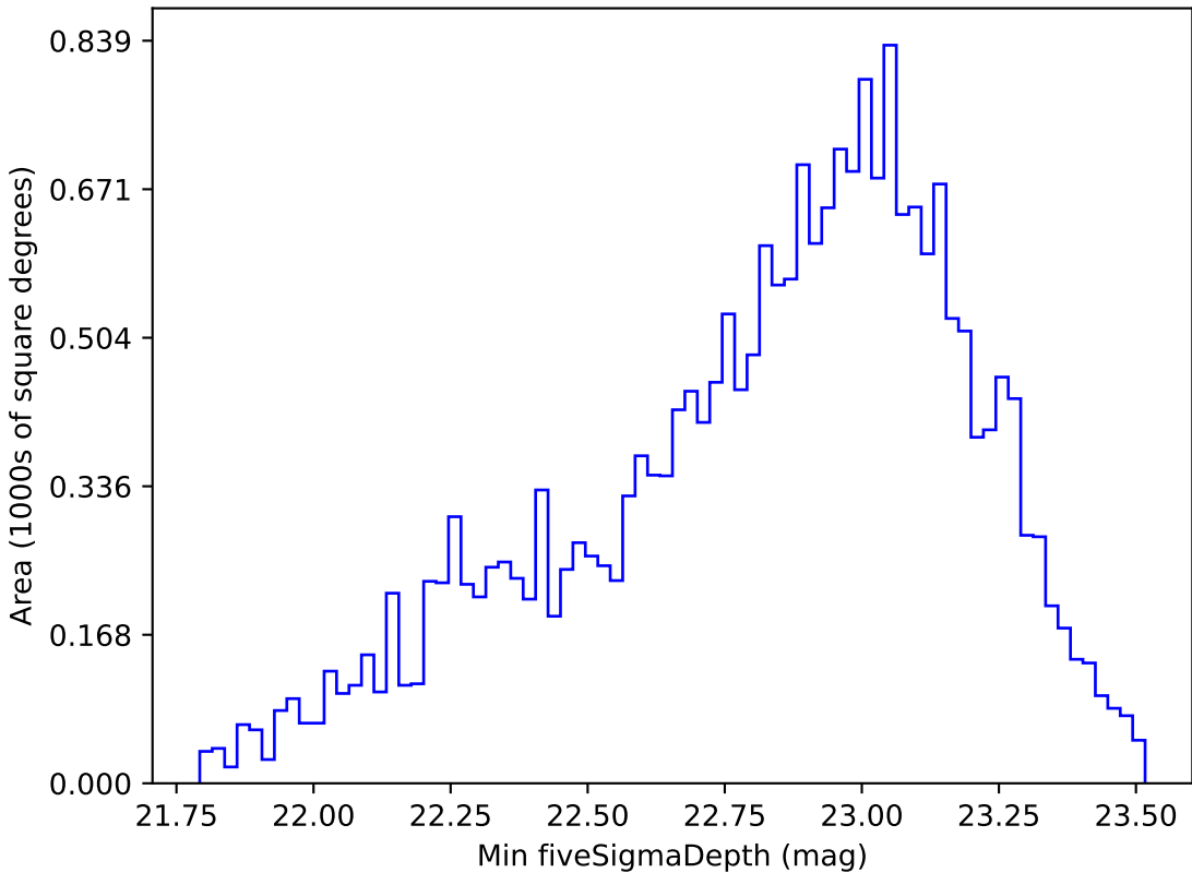
extra_ss_neo2_v3.4_10yrs Yr 1 u band: Min fiveSigmaDepth
