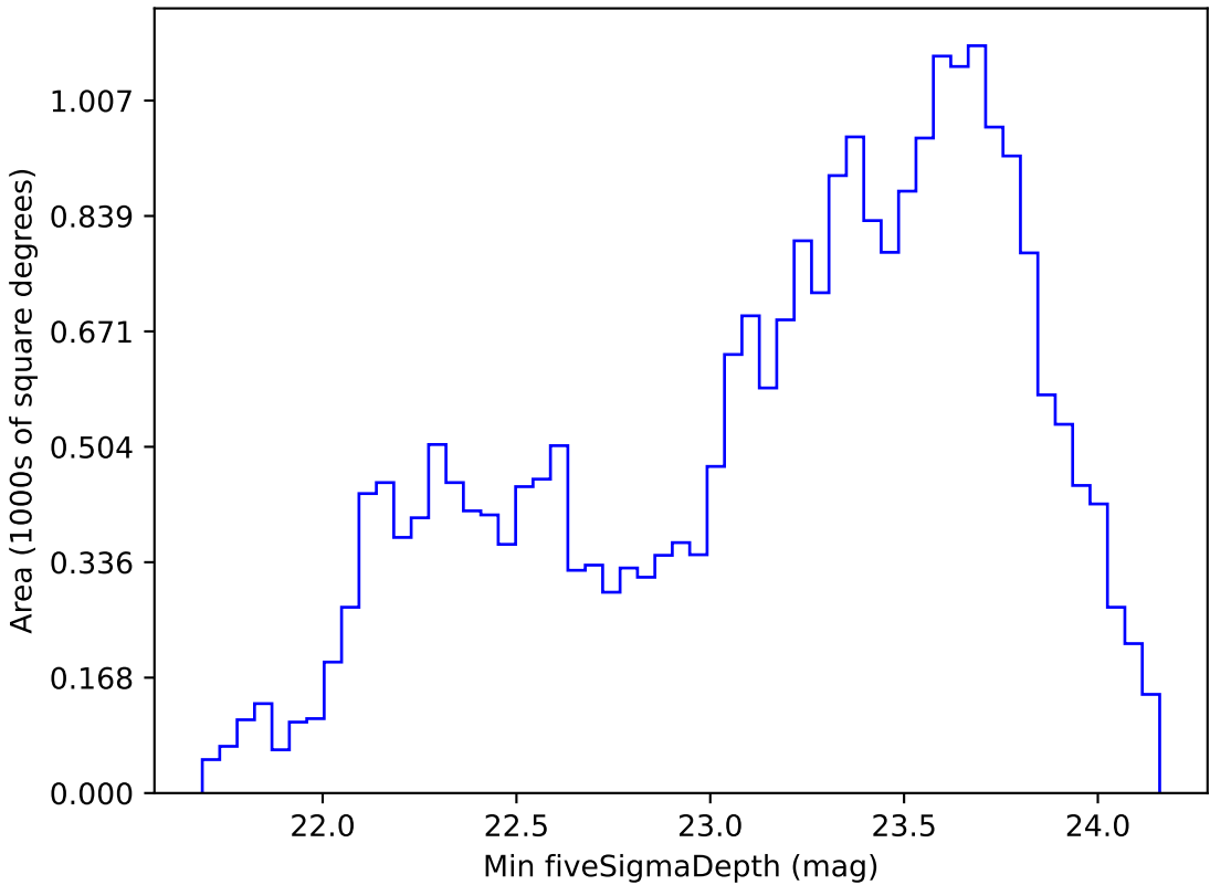
extra_ss_neo2_v3.4_10yrs Yr 1 r band: Min fiveSigmaDepth
