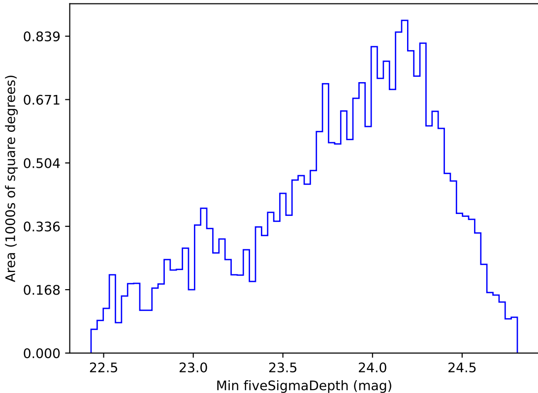
extra_ss_neo2_v3.4_10yrs Yr 1 g band: Min fiveSigmaDepth
