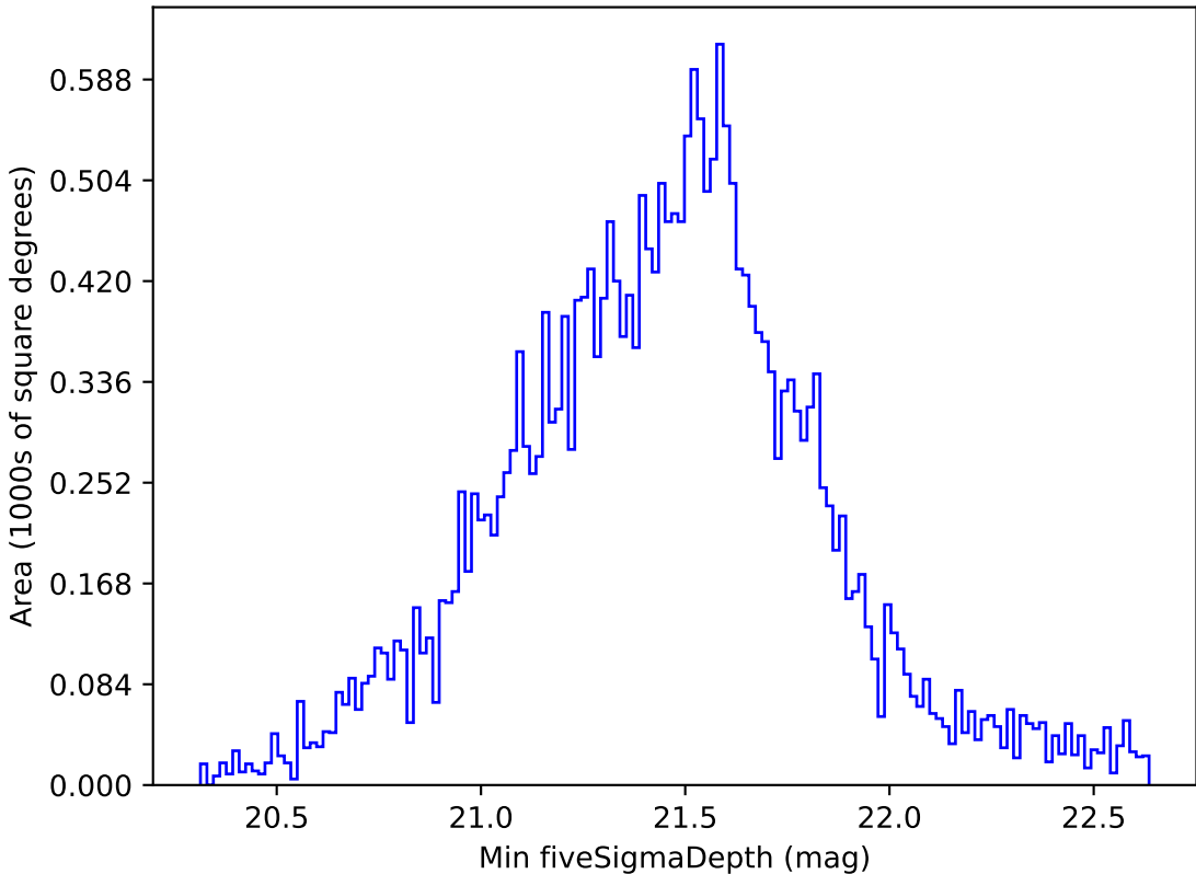
extra_ss_neo2_v3.4_10yrs Yr 1 all bands: Min fiveSigmaDepth
