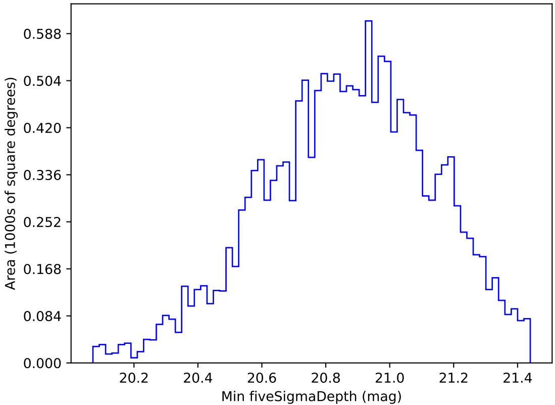
extra_ss_neo2_v3.4_10yrs WFD y band: Min fiveSigmaDepth
