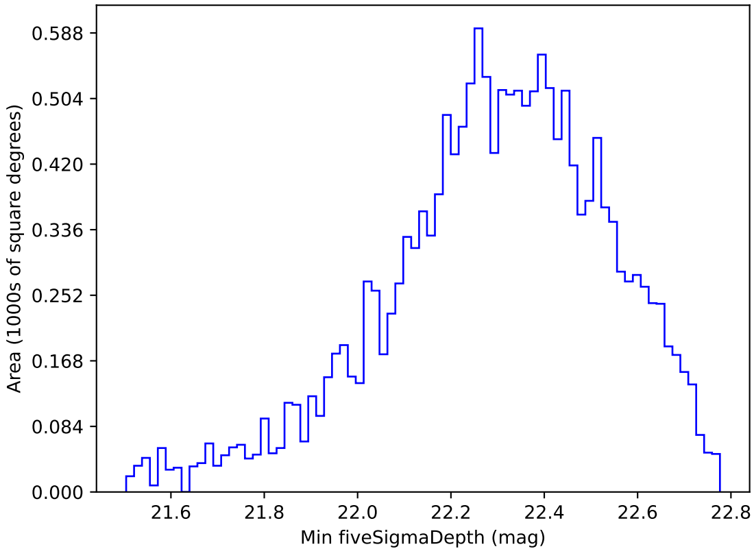
extra_ss_neo2_v3.4_10yrs WFD u band: Min fiveSigmaDepth
