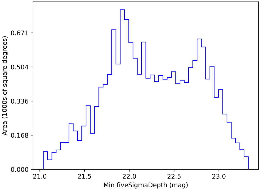
extra_ss_neo2_v3.4_10yrs WFD r band: Min fiveSigmaDepth
