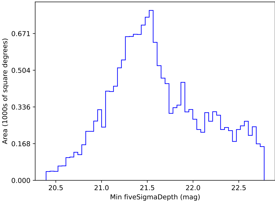
extra_ss_neo2_v3.4_10yrs WFD i band: Min fiveSigmaDepth
