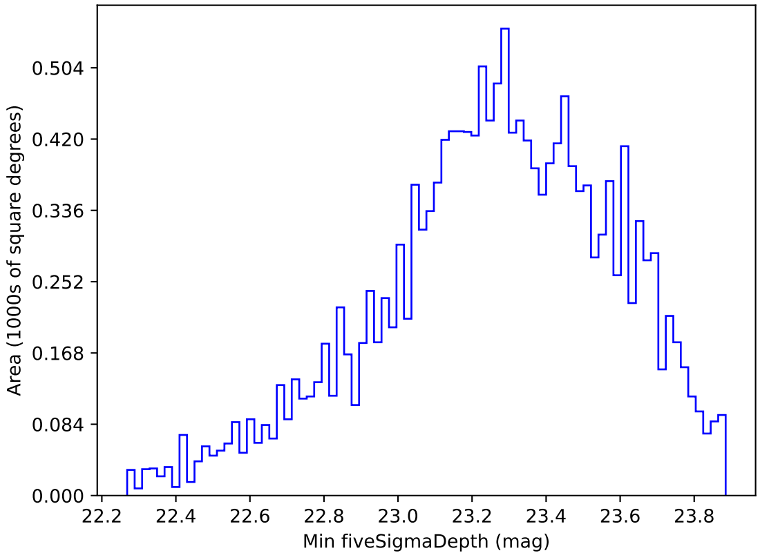
extra_ss_neo2_v3.4_10yrs WFD g band: Min fiveSigmaDepth
