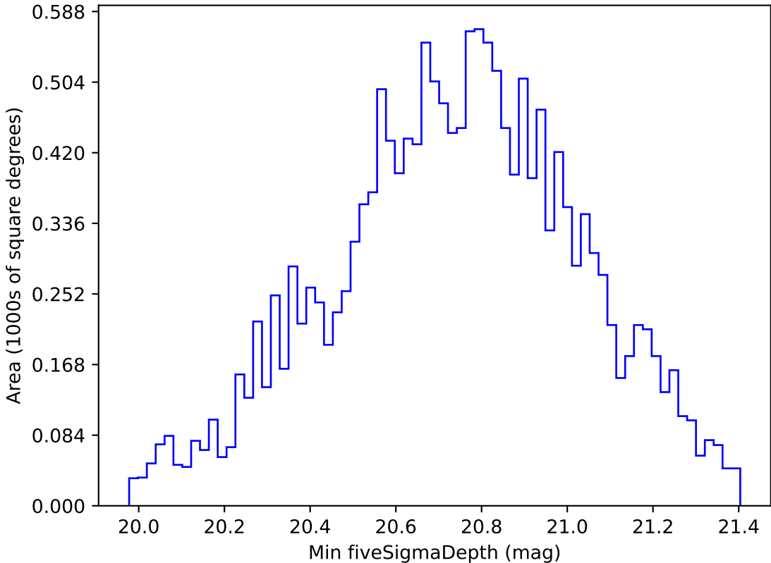
extra_ss_neo2_v3.4_10yrs WFD all bands: Min fiveSigmaDepth
