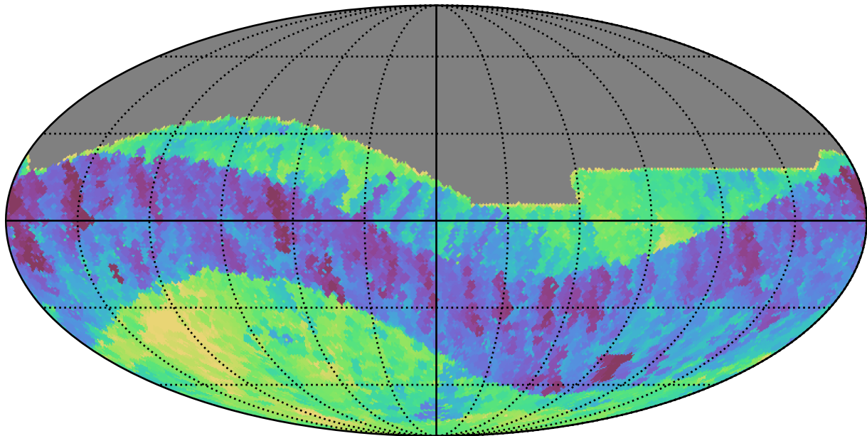
extra_ss_neo2_v3.4_10yrs All sky z band: Min fiveSigmaDepth
