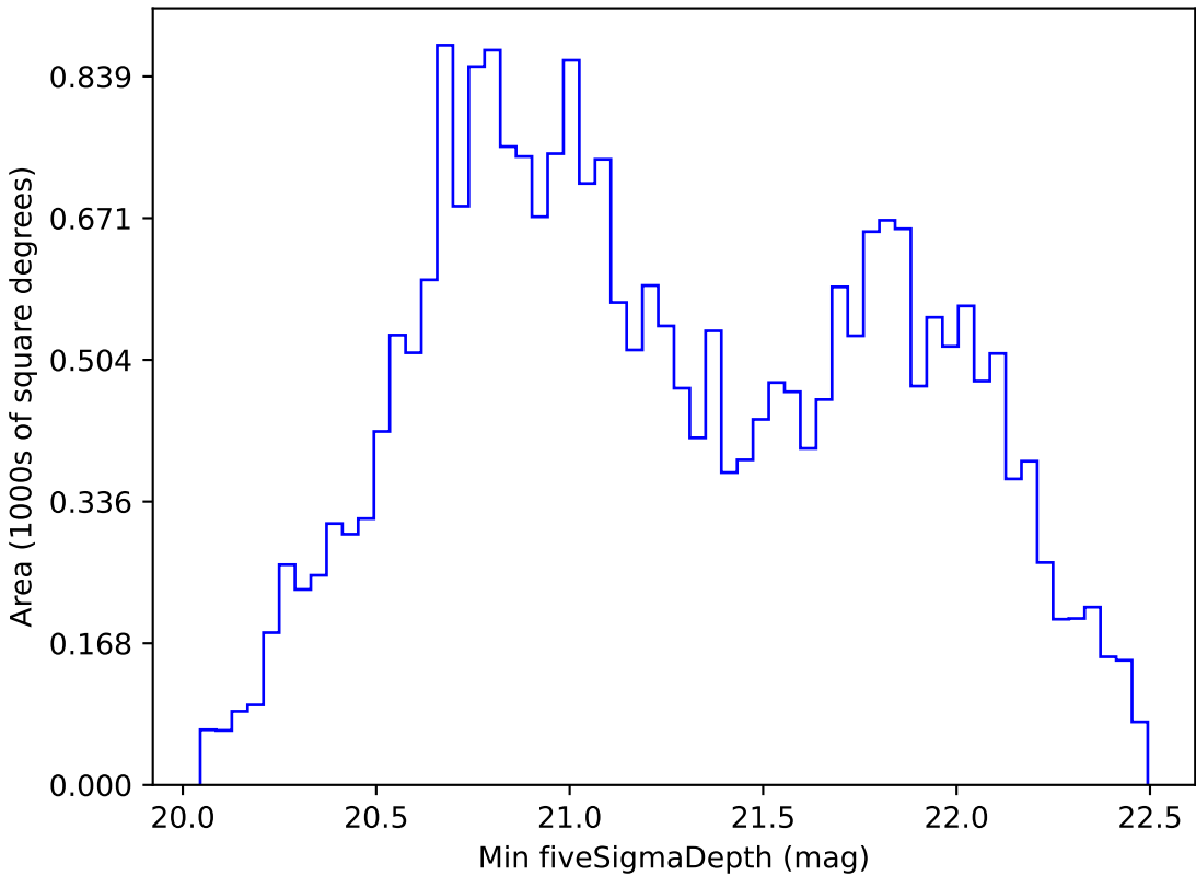
extra_ss_neo2_v3.4_10yrs All sky z band: Min fiveSigmaDepth
