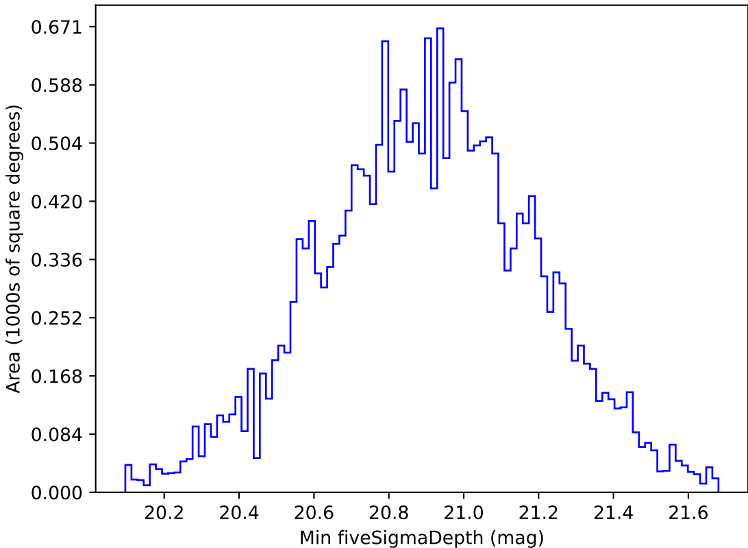
extra_ss_neo2_v3.4_10yrs All sky y band: Min fiveSigmaDepth
