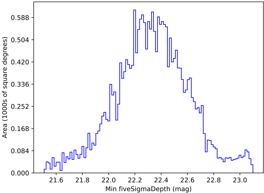
extra_ss_neo2_v3.4_10yrs All sky u band: Min fiveSigmaDepth
