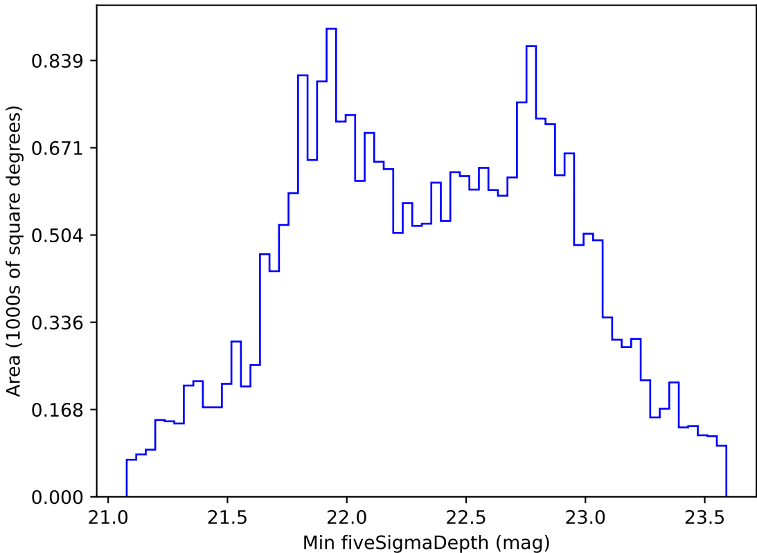
extra_ss_neo2_v3.4_10yrs All sky r band: Min fiveSigmaDepth
