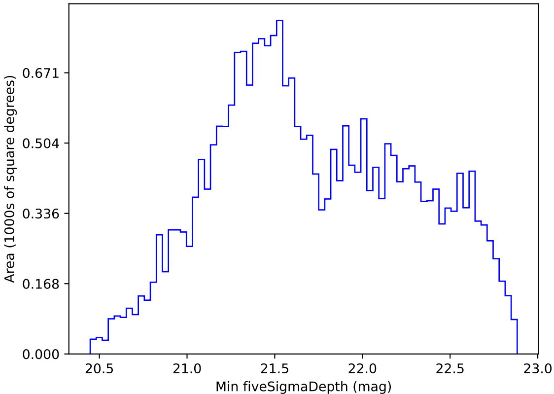
extra_ss_neo2_v3.4_10yrs All sky i band: Min fiveSigmaDepth
