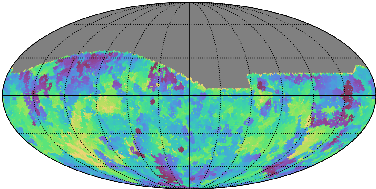
extra_ss_neo2_v3.4_10yrs All sky g band: Min fiveSigmaDepth
