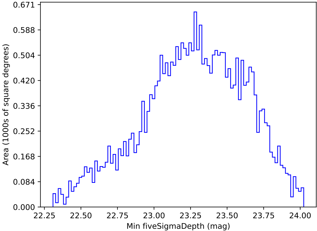
extra_ss_neo2_v3.4_10yrs All sky g band: Min fiveSigmaDepth
