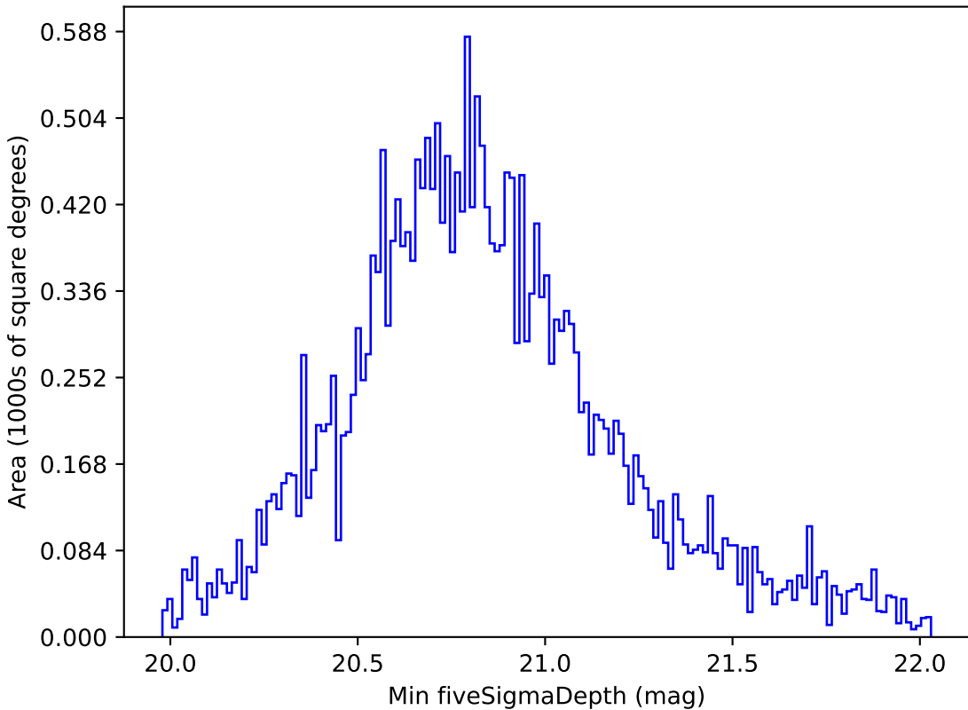
extra_ss_neo2_v3.4_10yrs All sky all bands: Min fiveSigmaDepth
