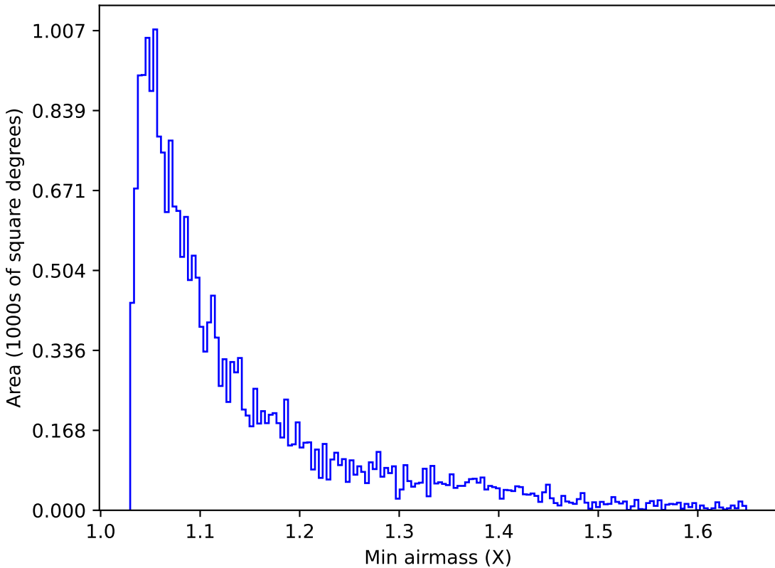
extra_ss_neo2_v3.4_10yrs Yr 1 u band: Min airmass
