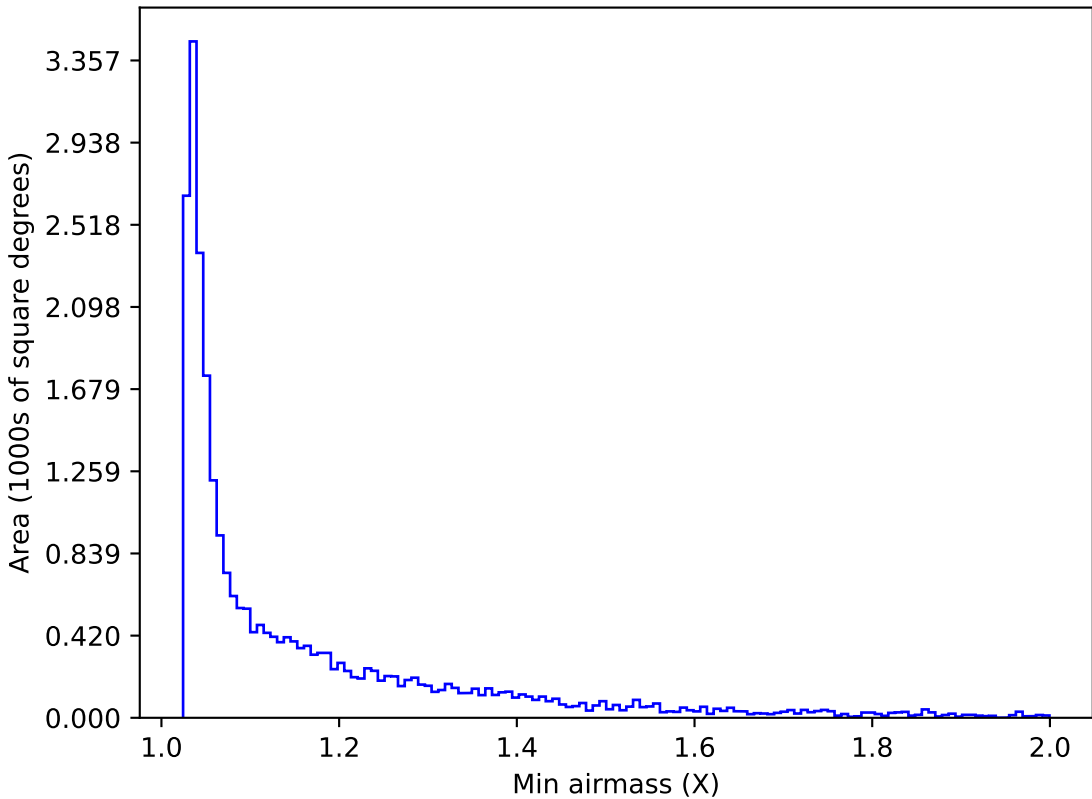
extra_ss_neo2_v3.4_10yrs Yr 1 i band: Min airmass
