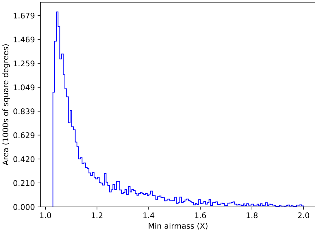
extra_ss_neo2_v3.4_10yrs Yr 1 g band: Min airmass
