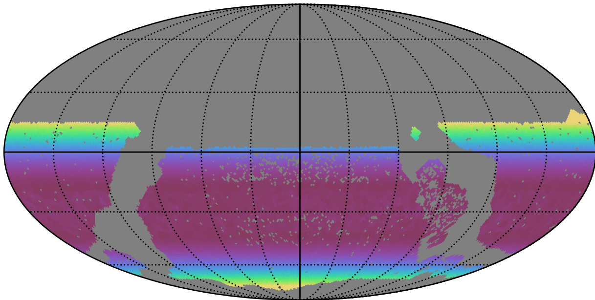
extra_ss_neo2_v3.4_10yrs WFD y band: Min airmass
