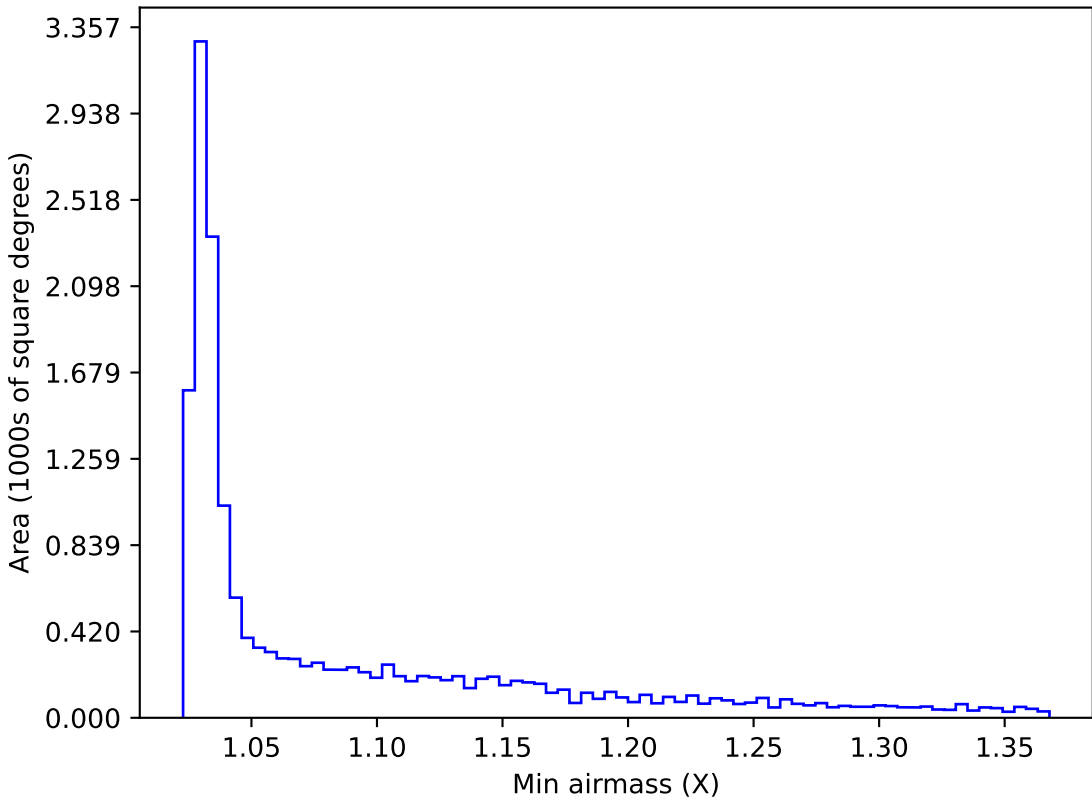
extra_ss_neo2_v3.4_10yrs WFD y band: Min airmass
