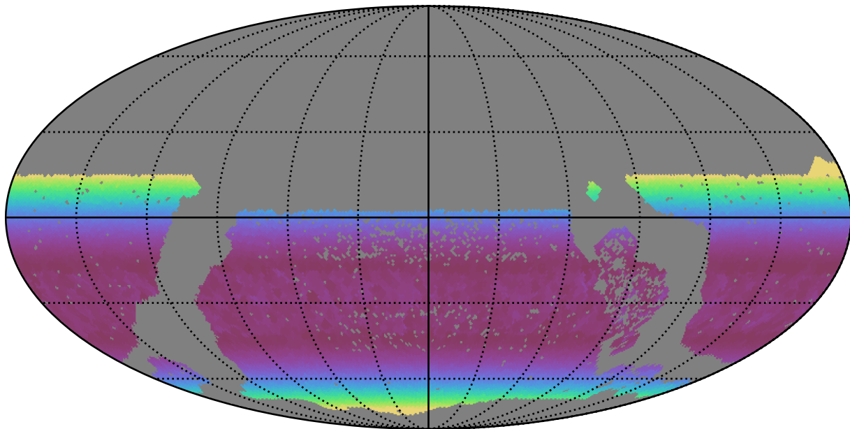
extra_ss_neo2_v3.4_10yrs WFD u band: Min airmass
