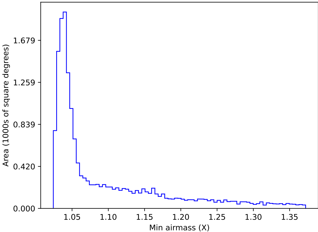
extra_ss_neo2_v3.4_10yrs WFD u band: Min airmass
