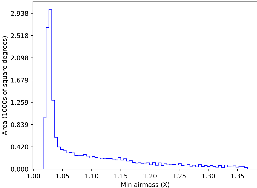
extra_ss_neo2_v3.4_10yrs WFD r band: Min airmass
