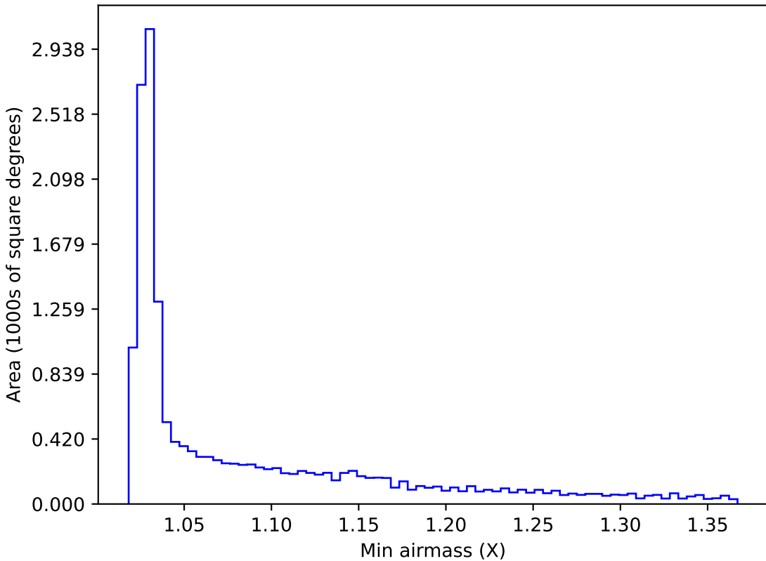
extra_ss_neo2_v3.4_10yrs WFD i band: Min airmass
