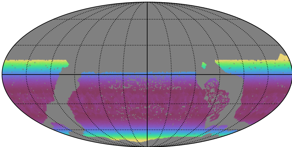
extra_ss_neo2_v3.4_10yrs WFD g band: Min airmass
