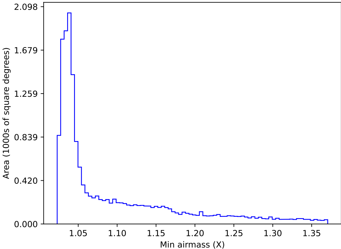
extra_ss_neo2_v3.4_10yrs WFD g band: Min airmass
