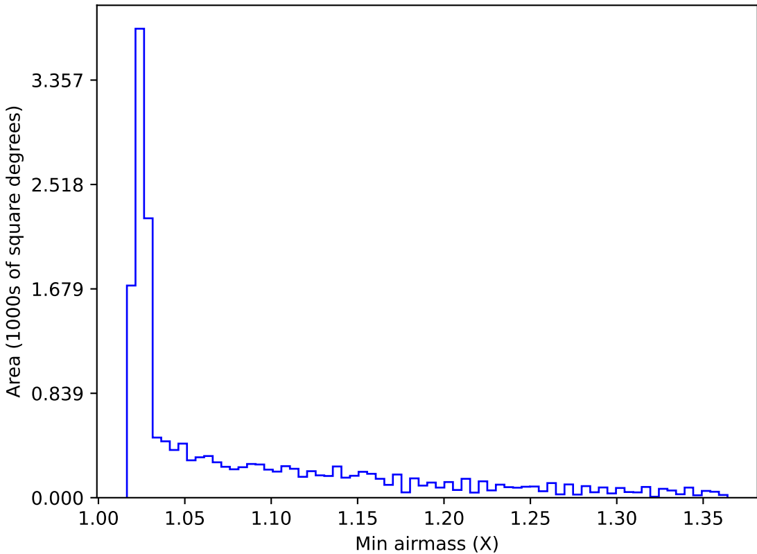
extra_ss_neo2_v3.4_10yrs WFD all bands: Min airmass
