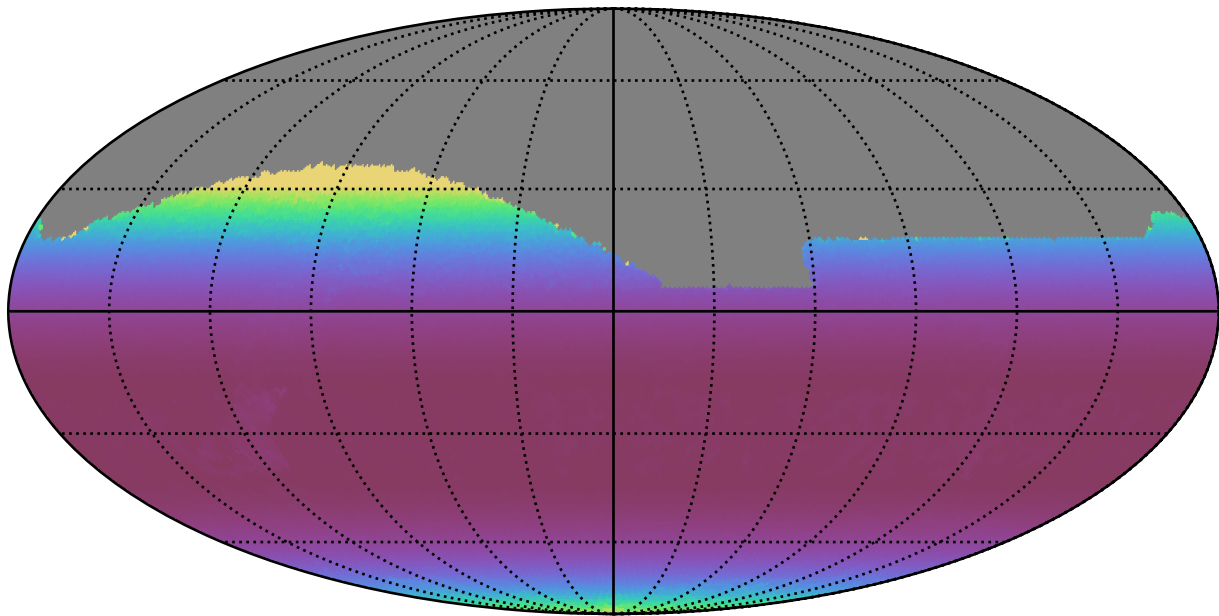
extra_ss_neo2_v3.4_10yrs All sky z band: Min airmass
