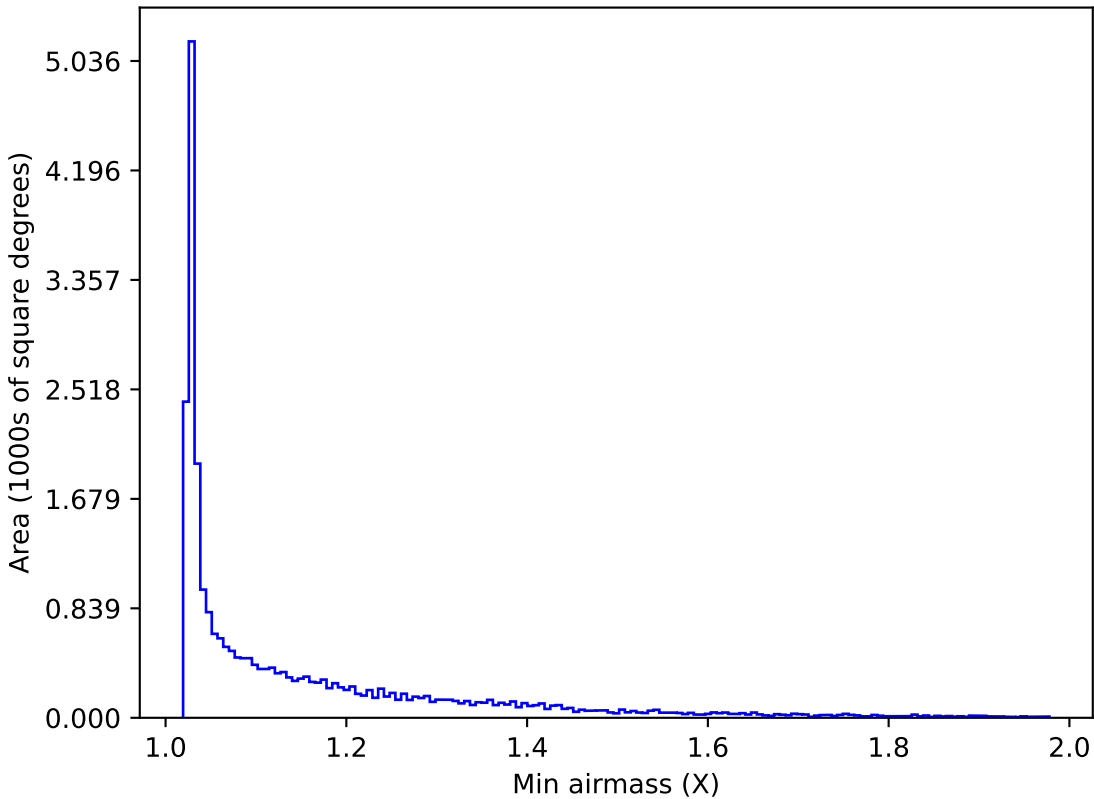
extra_ss_neo2_v3.4_10yrs All sky z band: Min airmass
