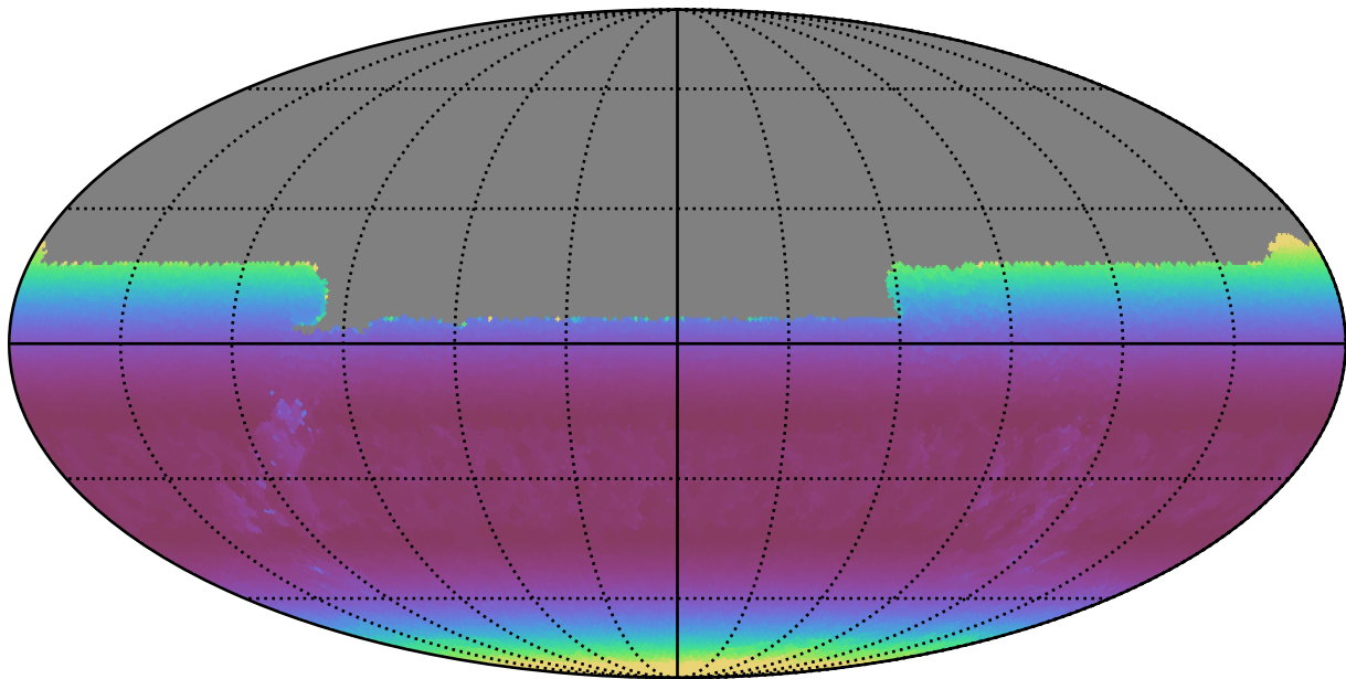
extra_ss_neo2_v3.4_10yrs All sky u band: Min airmass
