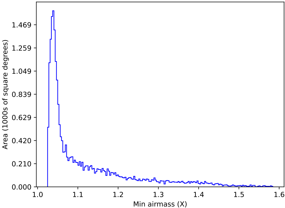
extra_ss_neo2_v3.4_10yrs All sky u band: Min airmass
