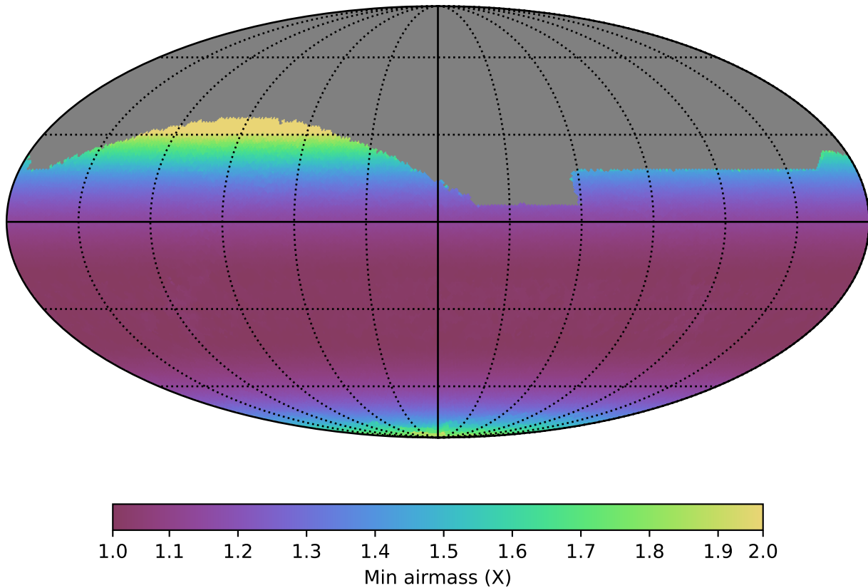
extra_ss_neo2_v3.4_10yrs All sky r band: Min airmass
