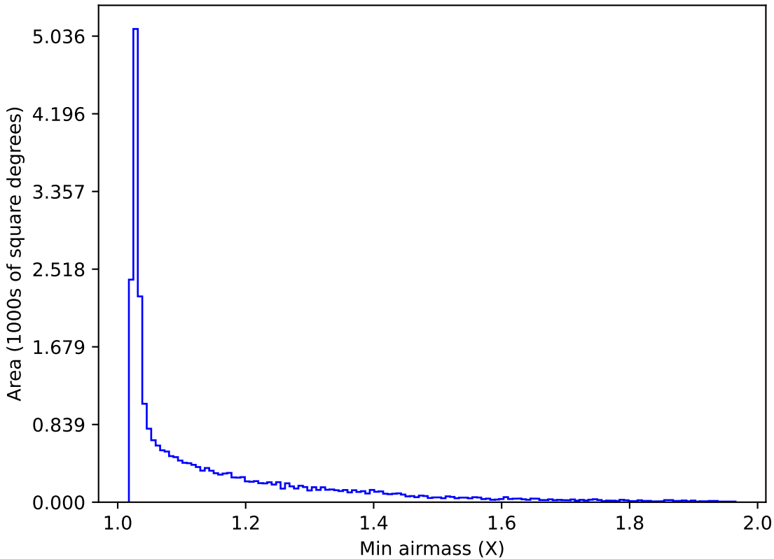
extra_ss_neo2_v3.4_10yrs All sky r band: Min airmass
