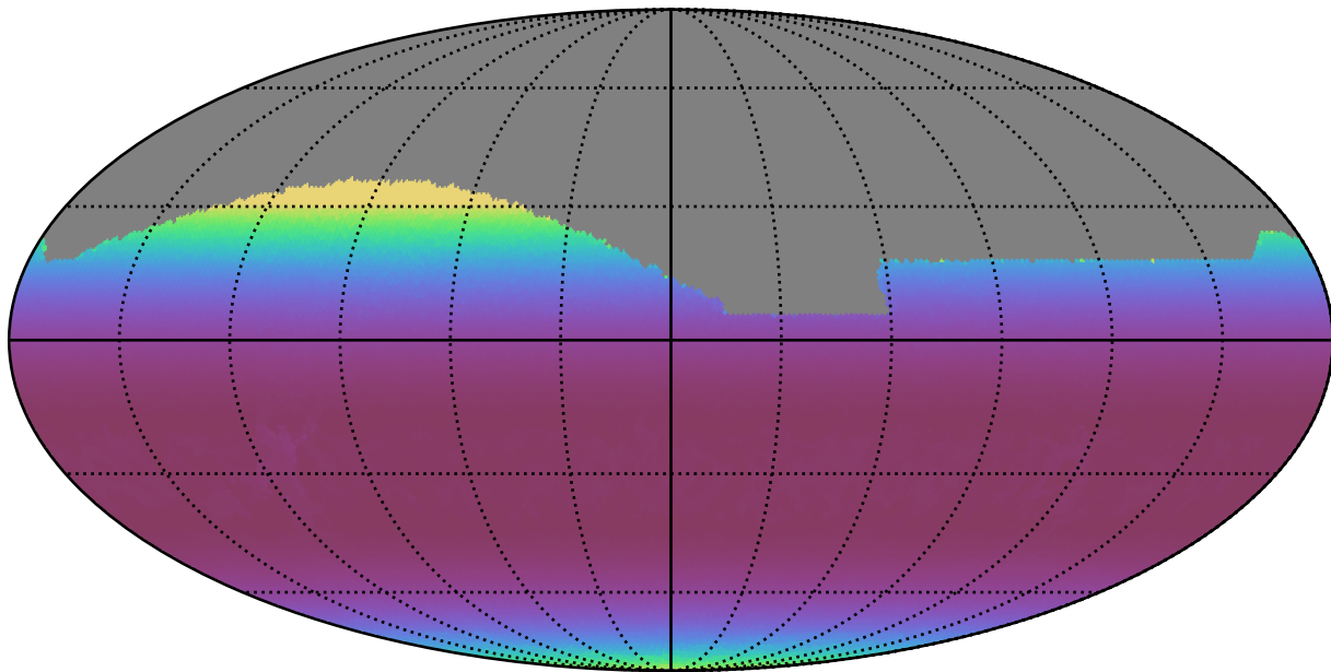
extra_ss_neo2_v3.4_10yrs All sky i band: Min airmass
