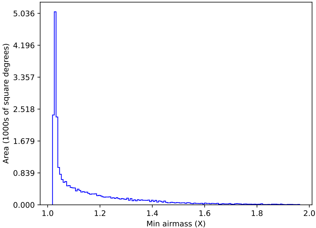
extra_ss_neo2_v3.4_10yrs All sky i band: Min airmass
