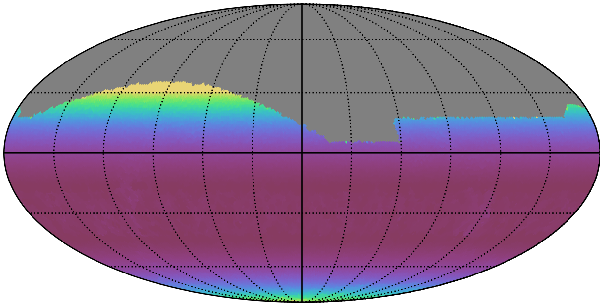
extra_ss_neo2_v3.4_10yrs All sky g band: Min airmass
