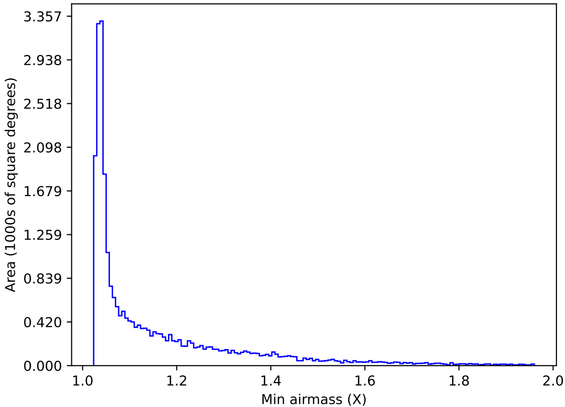
extra_ss_neo2_v3.4_10yrs All sky g band: Min airmass
